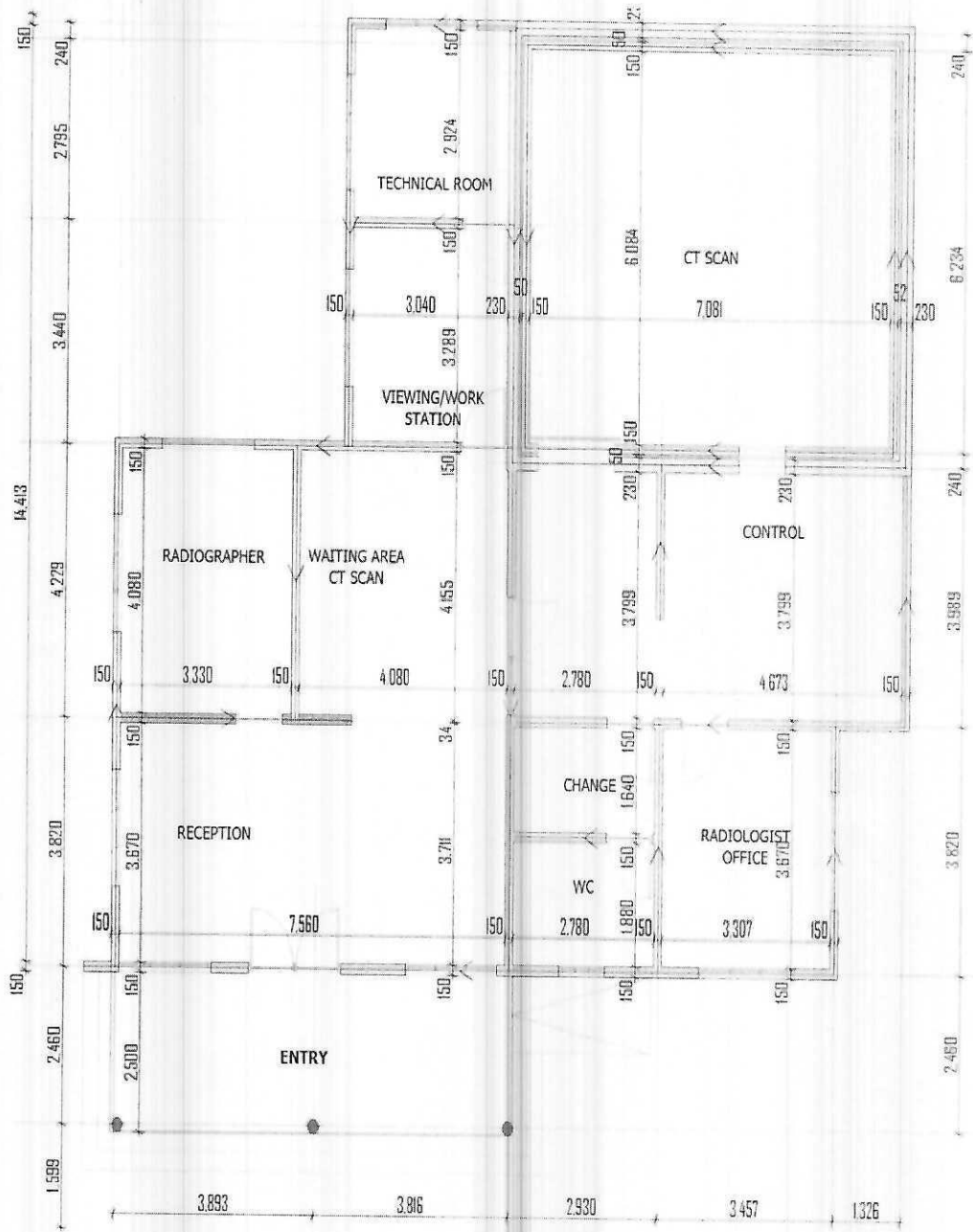
PROPOSED CT SCAN BUILDING
